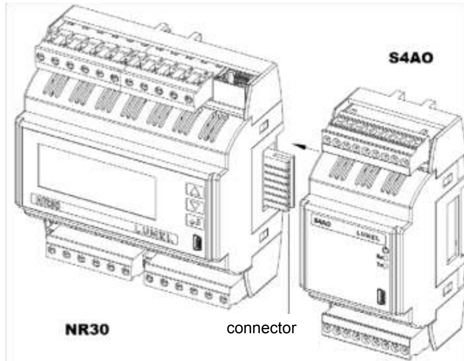
Fig.7. Connecting blocks using the side connector
