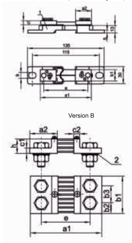
Fig.1. Fixing dimensions of shunts 1 - isolating base, 2 - round spring washer.
