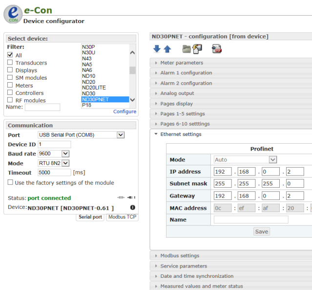
Fig.33. View of program window: a) eCon, b) firmware upgrade
