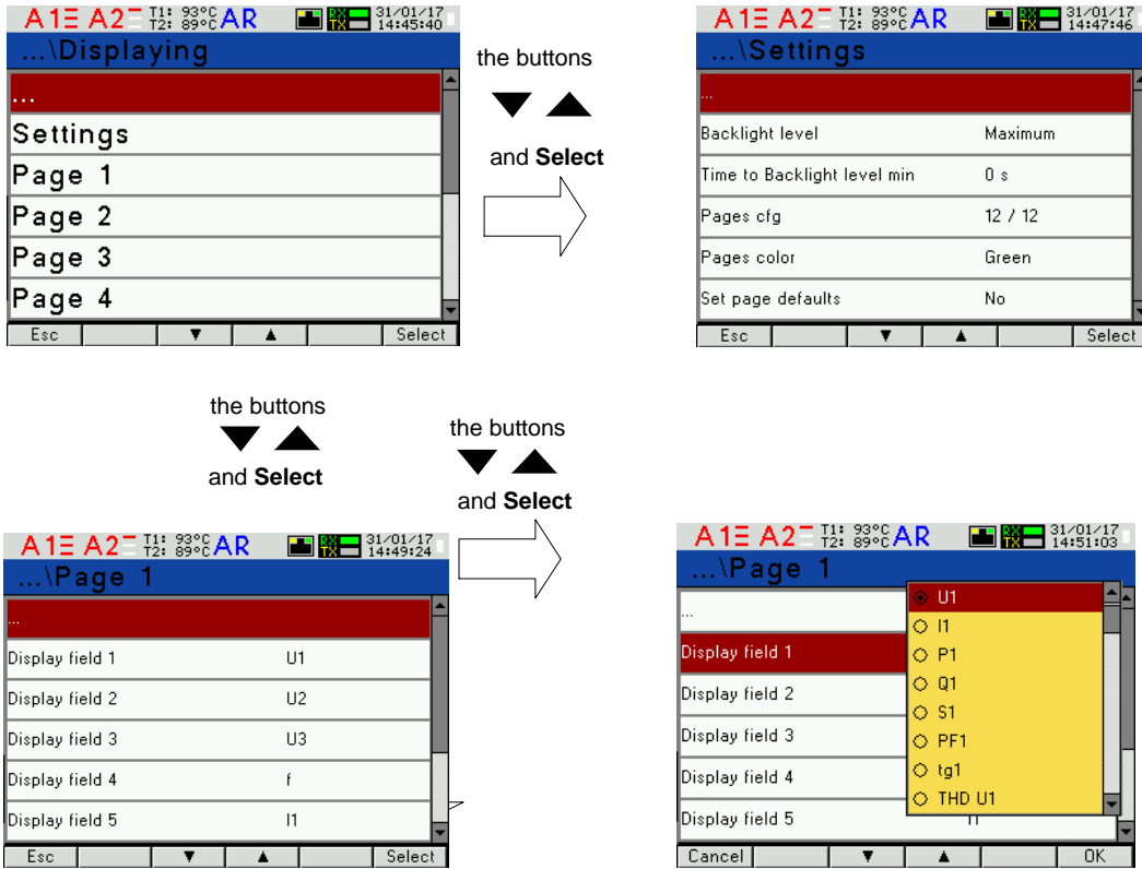
Fig.19. Screens of Displaying group
