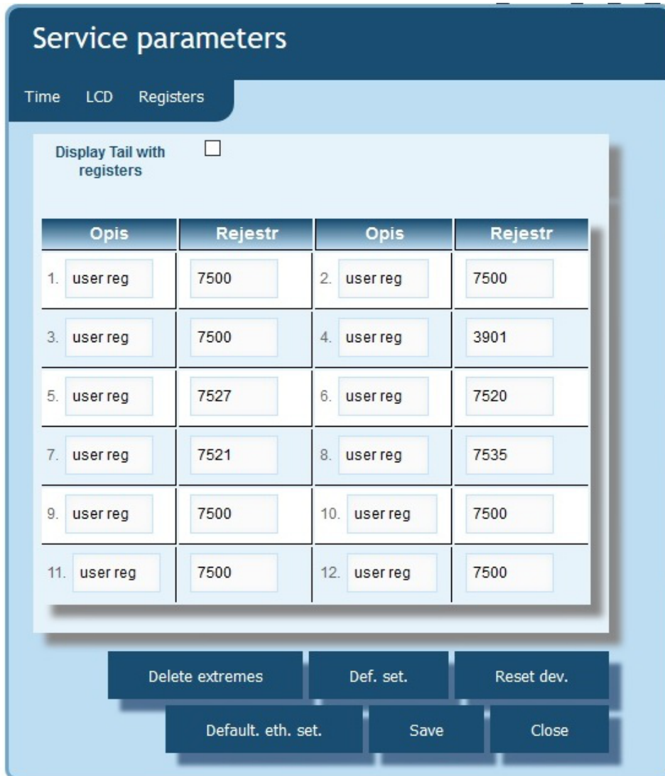
Fig. 9. View of the window to configure the group of our own registers
