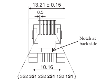
Meter Side RJ 12 Connection
