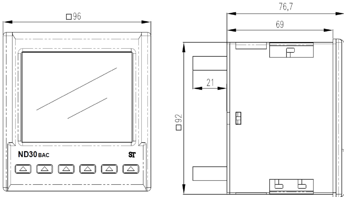
Fig. 3. Overall dimensions of the ND30BAC meter
