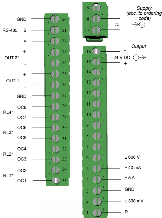
Fig. 1 Description of the terminal strip.
