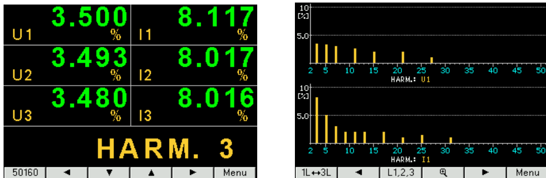
Fig. 16. Screens 11 and 12 - visualization of harmonics
