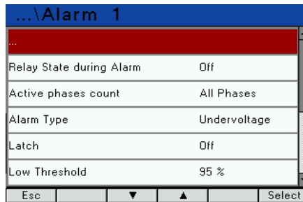
Fig. 20. Screens of Alarms mode
