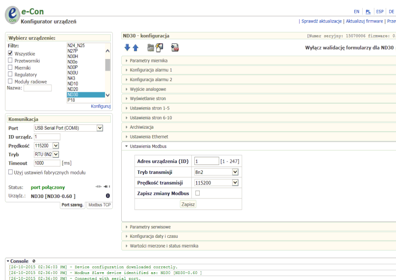
Fig.26. Program window view: a) eCon, b) software upgrade
