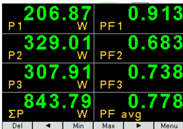
Fig. 11. Screen of meter measuring mode
