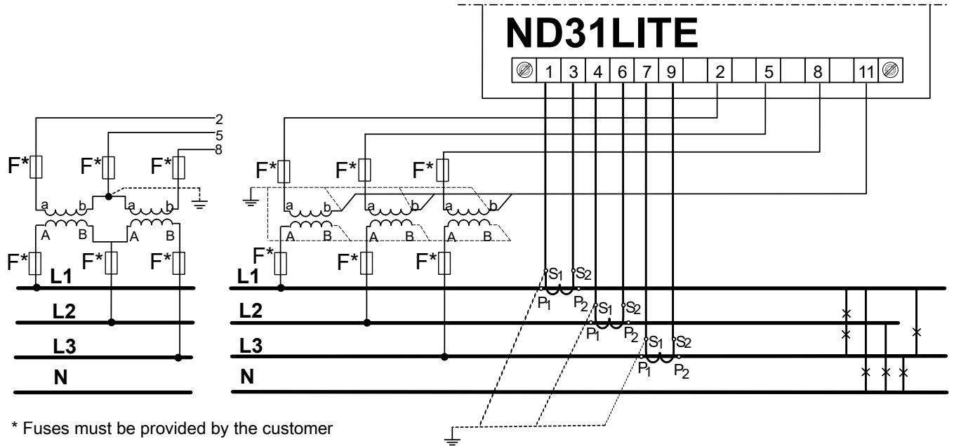
Fig.6.Connections of input signals in three-phase 4-wire network
