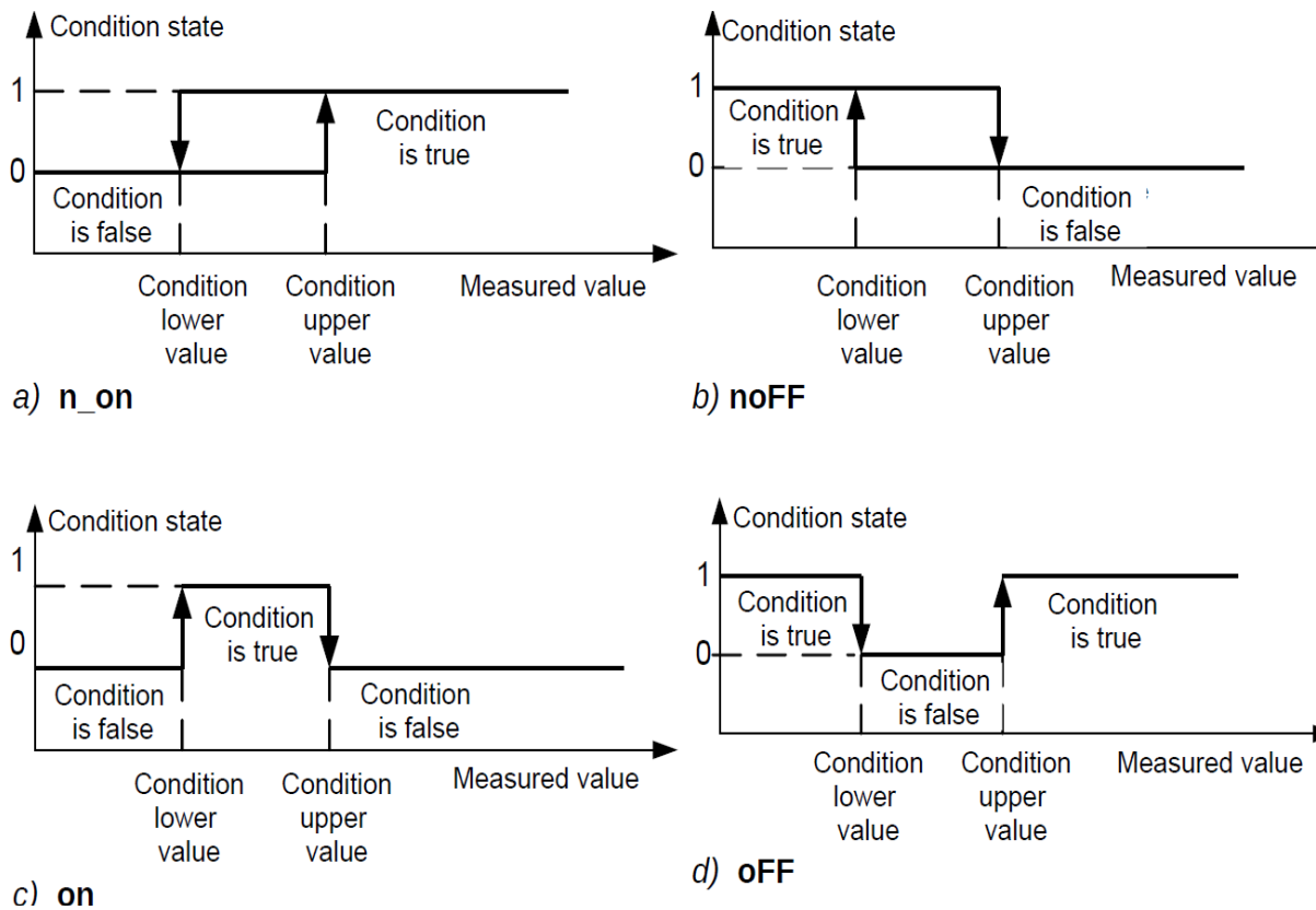
Fig. 21. Condition types: a) n_on b) noFF c) on d) OFF
