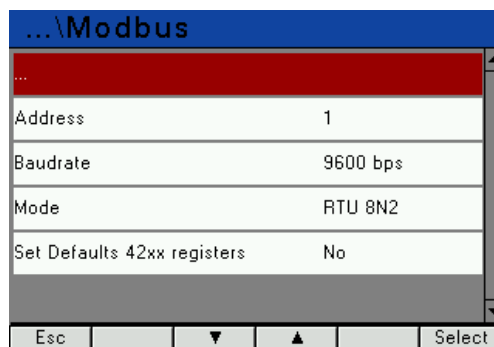
Fig.23. Screens of Modbus mode
